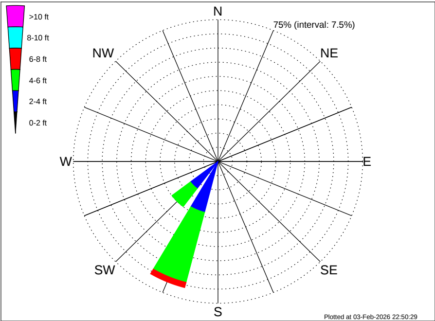
Angola Namibia CRS Luanda (BU-LU) Climatological WaveHeight Rose for January: 1979 - 2015
