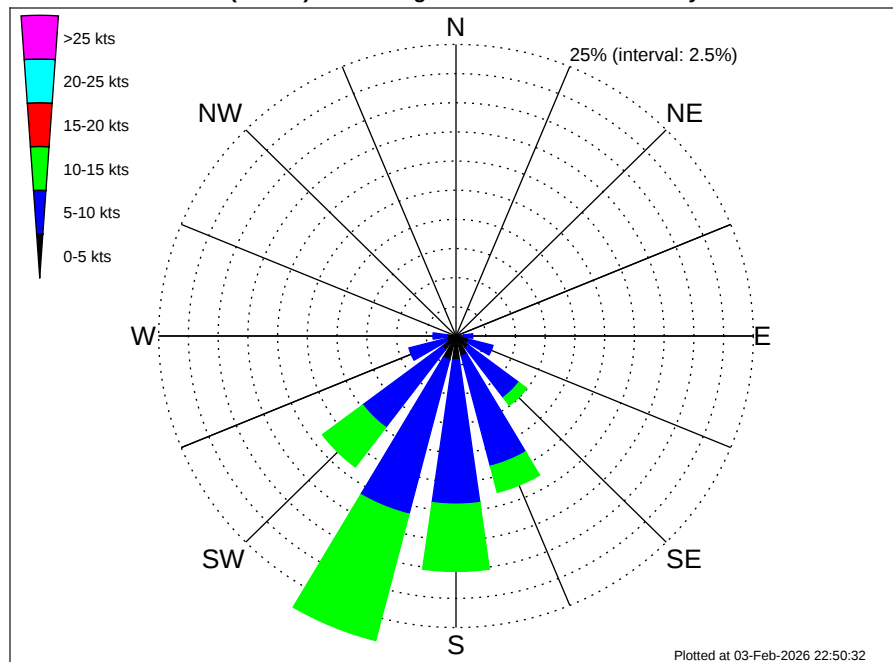
Angola Namibia CRS Luanda (BU-LU) Climatological Wind Rose for January: 1979 - 2015
