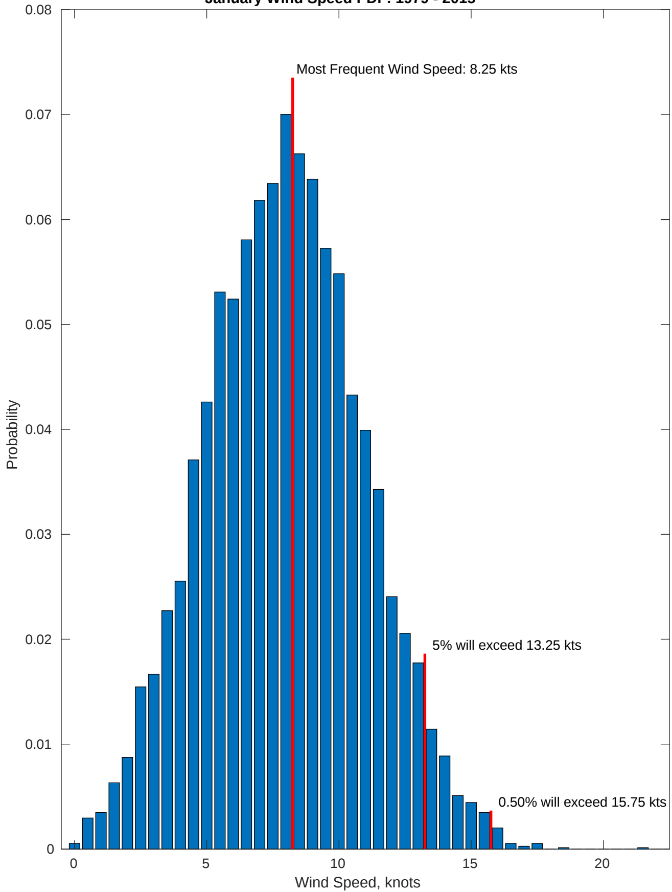
January Wind Speed PDF: 1979 - 2015
