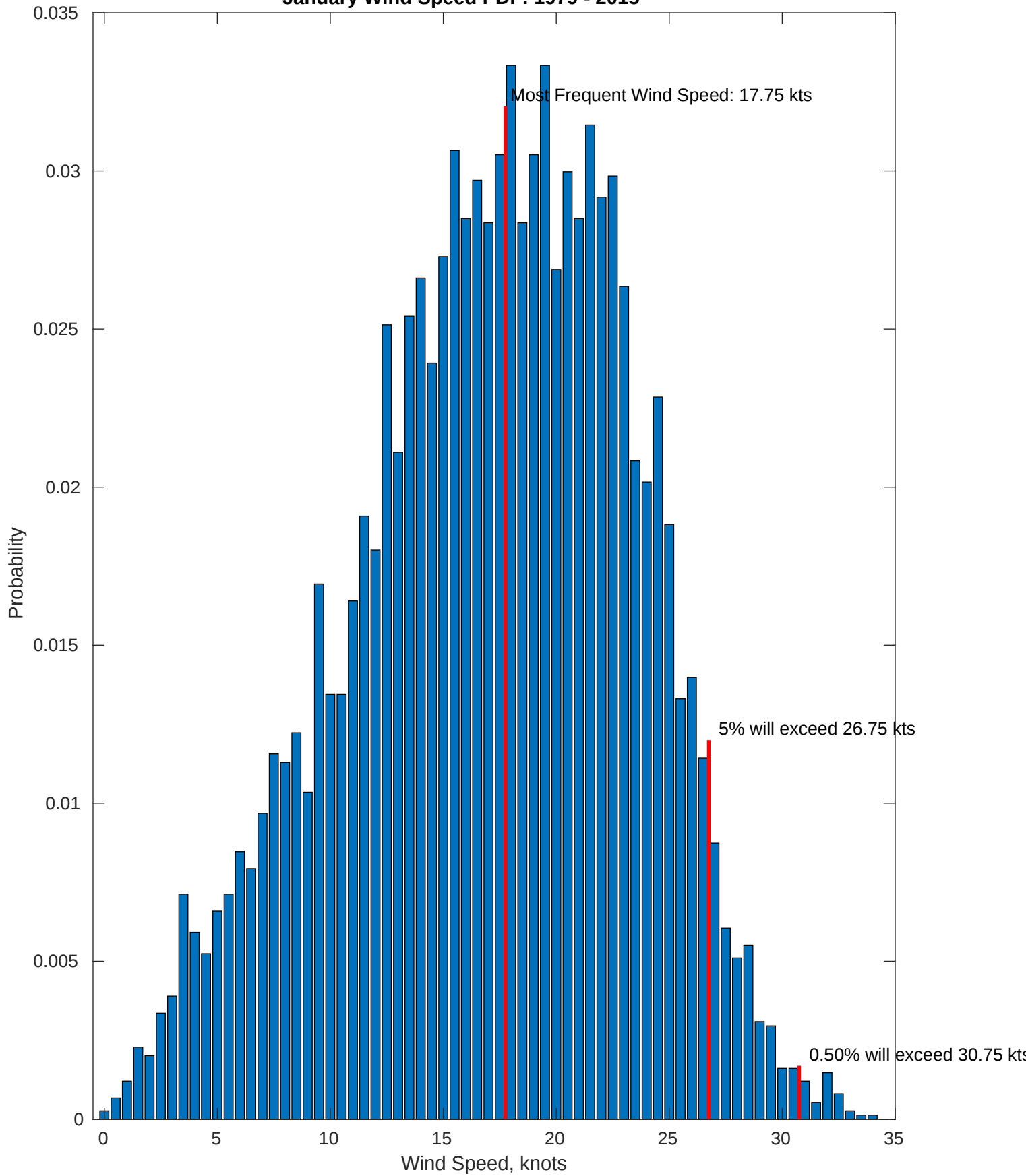
January Wind Speed PDF: 1979 - 2015
