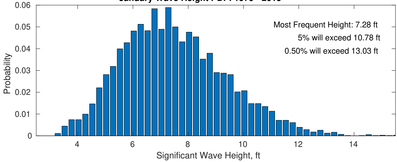
January Wave Height PDF: 1979 - 2015
