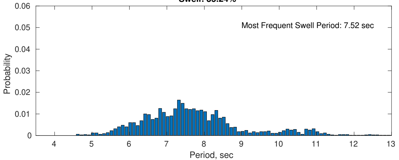
Swell: 35.24%
