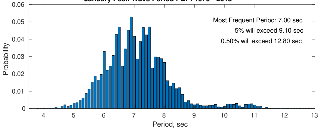
Wind-Sea: 64.76%
