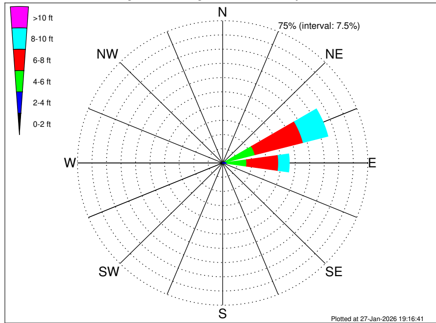
Aruba EBS Climatological WaveHeight Rose for January: 1979 - 2015
