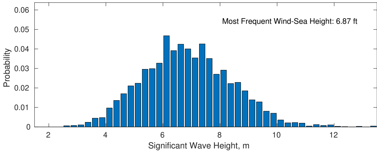
Wind-Sea: 64.76%
