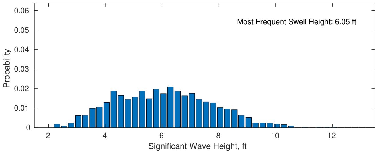
Swell: 35.24%
