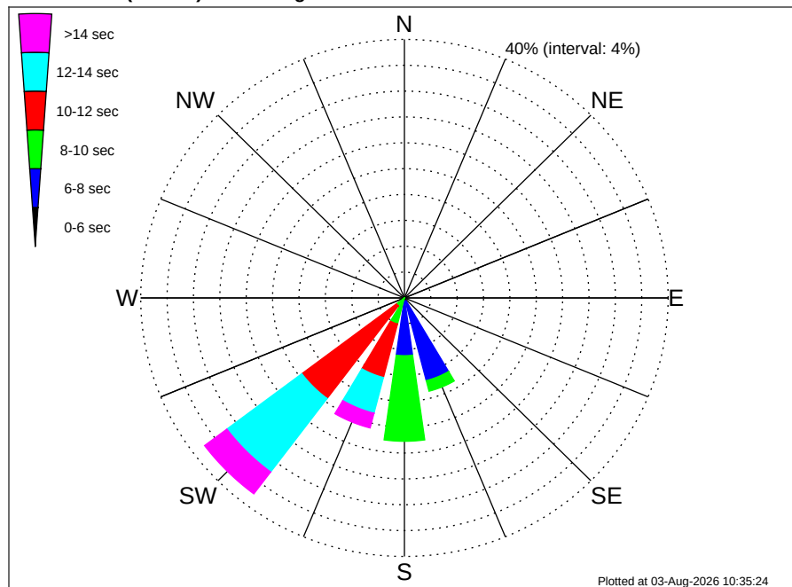
Namibia TE Luderitz (PEL-83) Climatological WavePeriod Rose for October: 1979 - 2015
