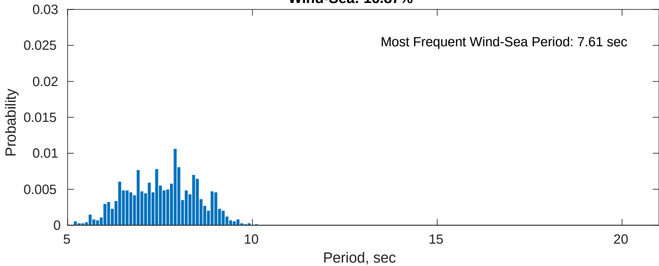
Wind-Sea: 16.87%
