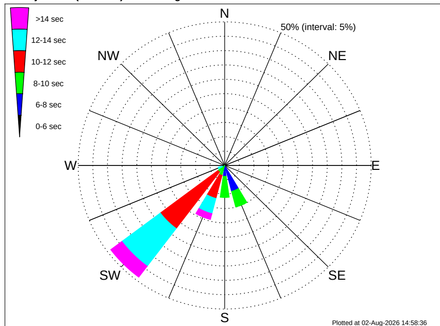
Namibia TE Oranjemund (PEL-104) Climatological WavePeriod Rose for October: 1979 - 2015
