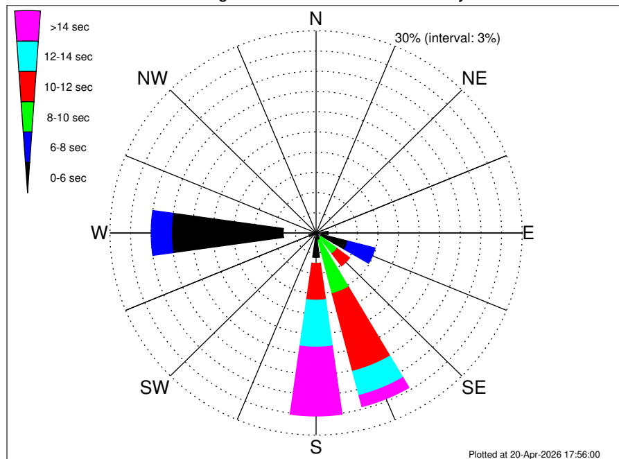
Petronas Oman Block 18 Climatological WavePeriod Rose for January: 1979 - 2015
