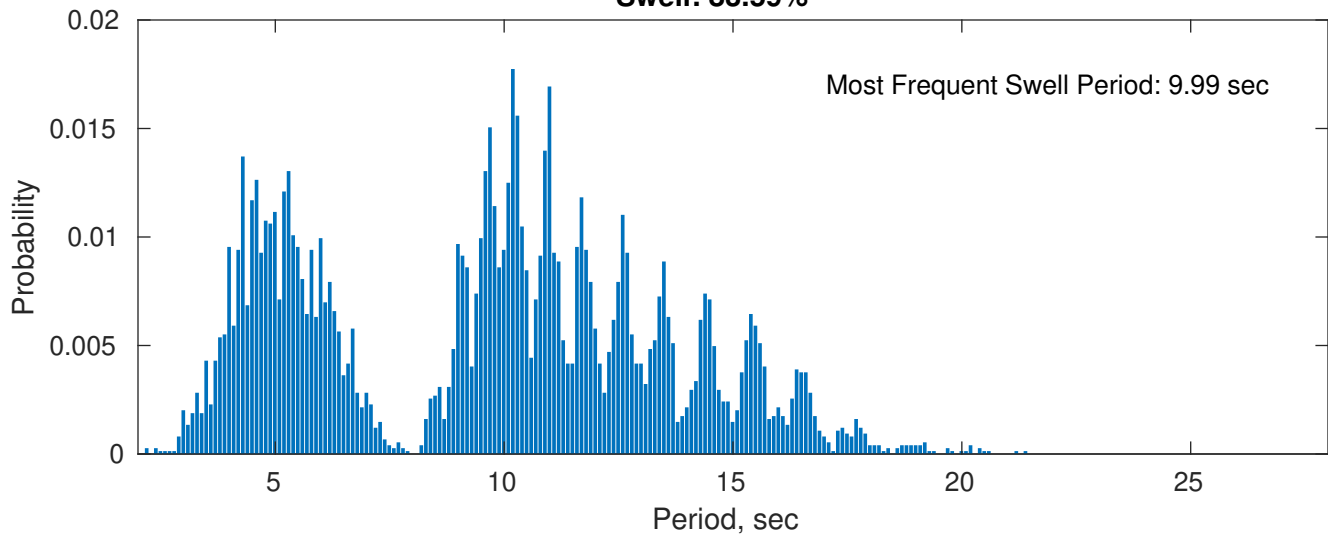
Swell: 83.59%
