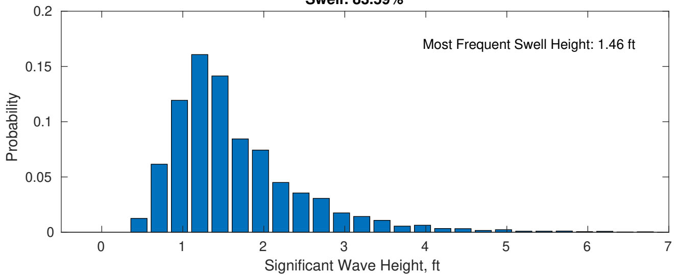
Swell: 83.59%
