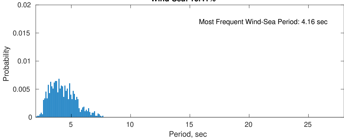
Wind-Sea: 16.41%
