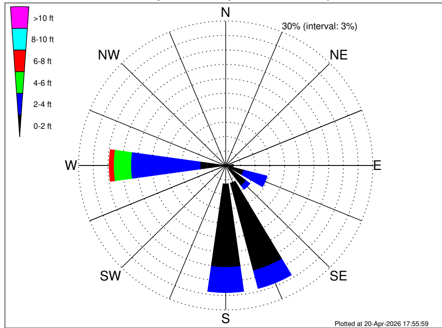
Petronas Oman Block 18 Climatological WaveHeight Rose for January: 1979 - 2015
