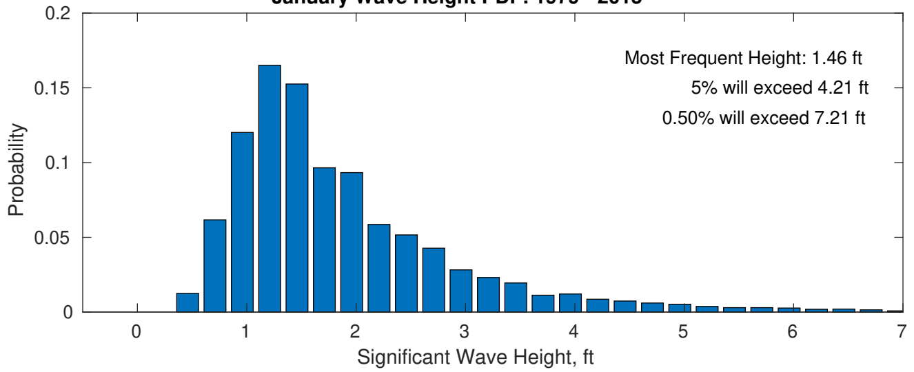
Wind-Sea: 16.41%
