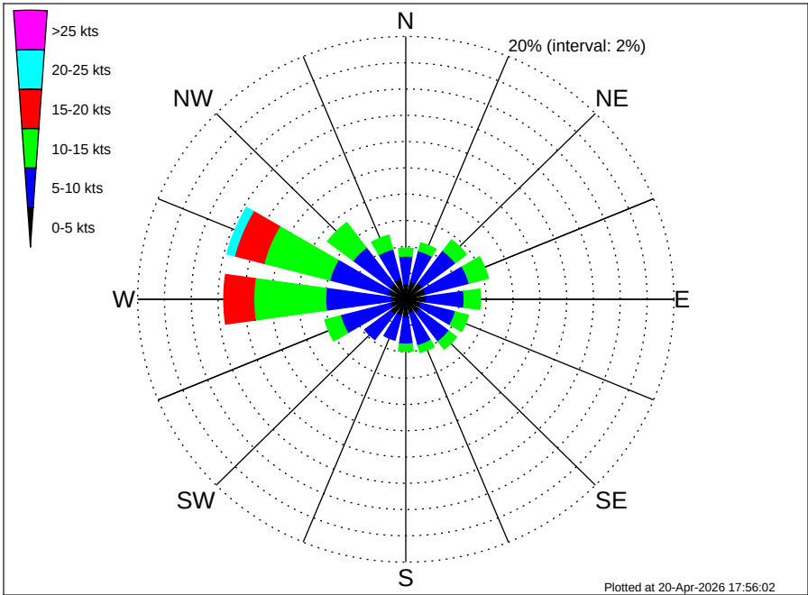
Petronas Oman Block 18 Climatological Wind Rose for January: 1979 - 2015
