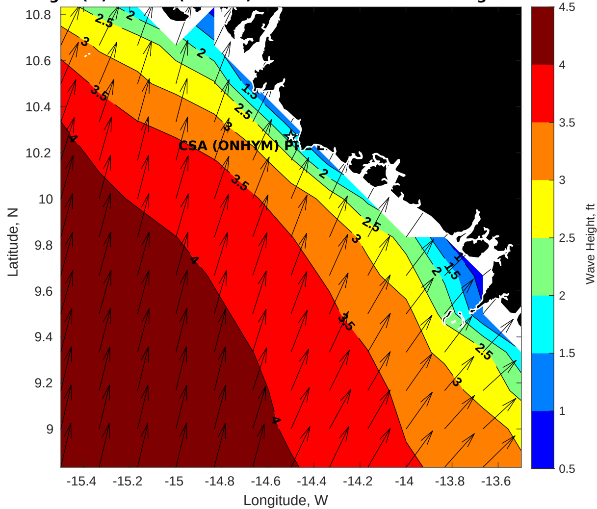
Wave Height (ft) for CSA (ONHYM) PPL EBS - Guinea at 23-Aug-2025 21:00:00
