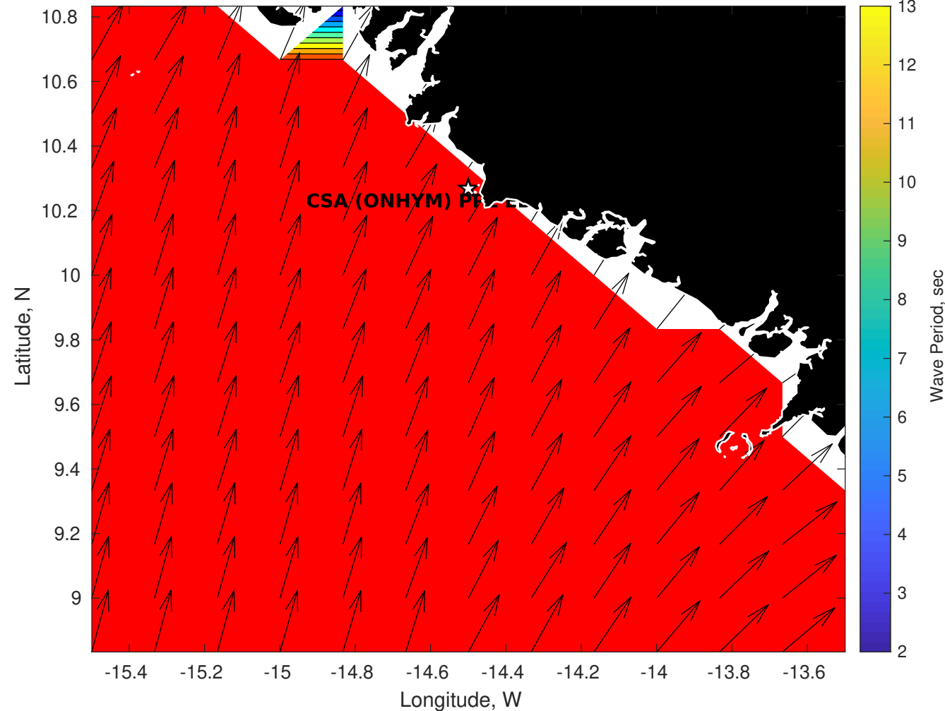
Wave Period (sec) for CSA (ONHYM) PPL EBS - Guinea at 23-Aug-2025 21:00:00
