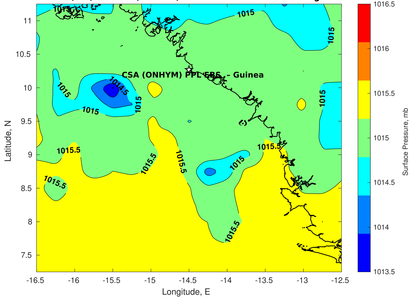
Surface Pressure (mb) for CSA (ONHYM) PPL EBS - Guinea at 24-Aug-2025 12:00:00
