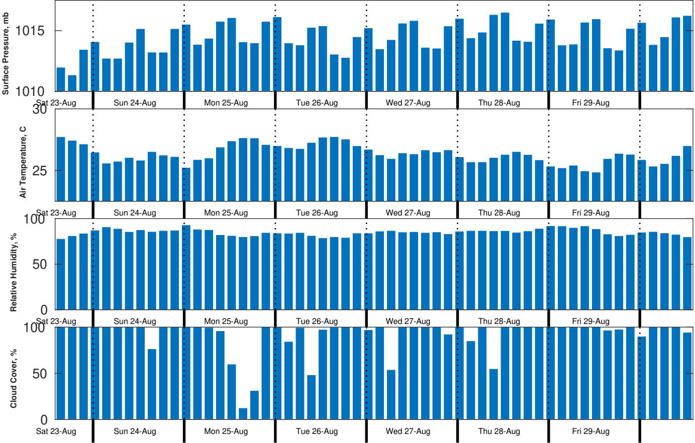
Met Forecast for CSA (ONHYM) PPL EBS - Guinea from 23-Aug-2025 12:00:00 to 30-Aug-2025 12:00:00
