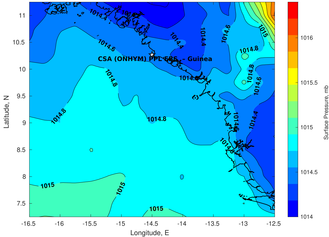
Surface Pressure (mb) for CSA (ONHYM) PPL EBS - Guinea at 23-Aug-2025 12:00:00
