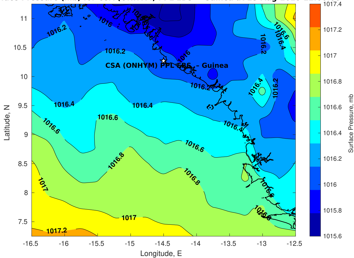
Surface Pressure (mb) for CSA (ONHYM) PPL EBS - Guinea at 25-Aug-2025 12:00:00
