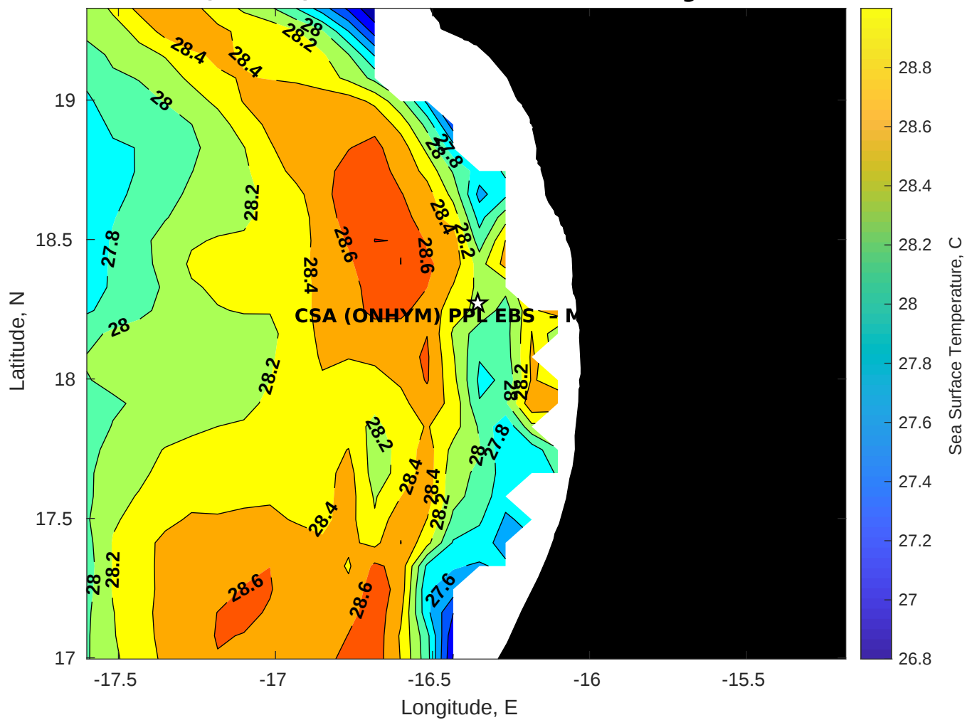
SST for CSA (ONHYM) PPL EBS - Mauritania at 23-Aug-2025 00:00:00
