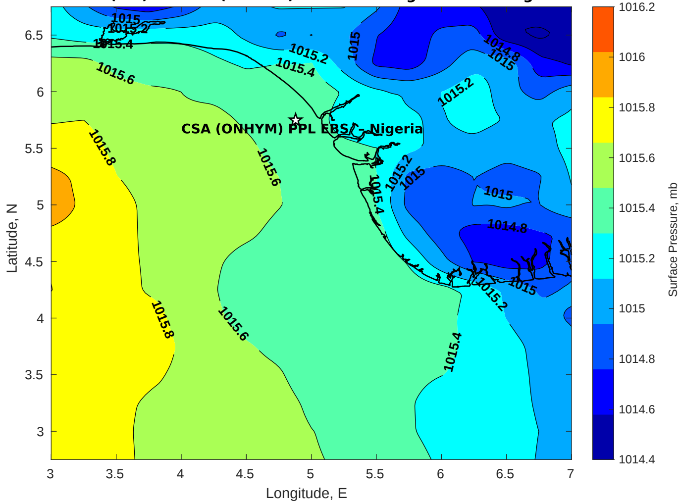
Surface Pressure (mb) for CSA (ONHYM) PPL EBS - Nigeria at 25-Aug-2025 12:00:00
