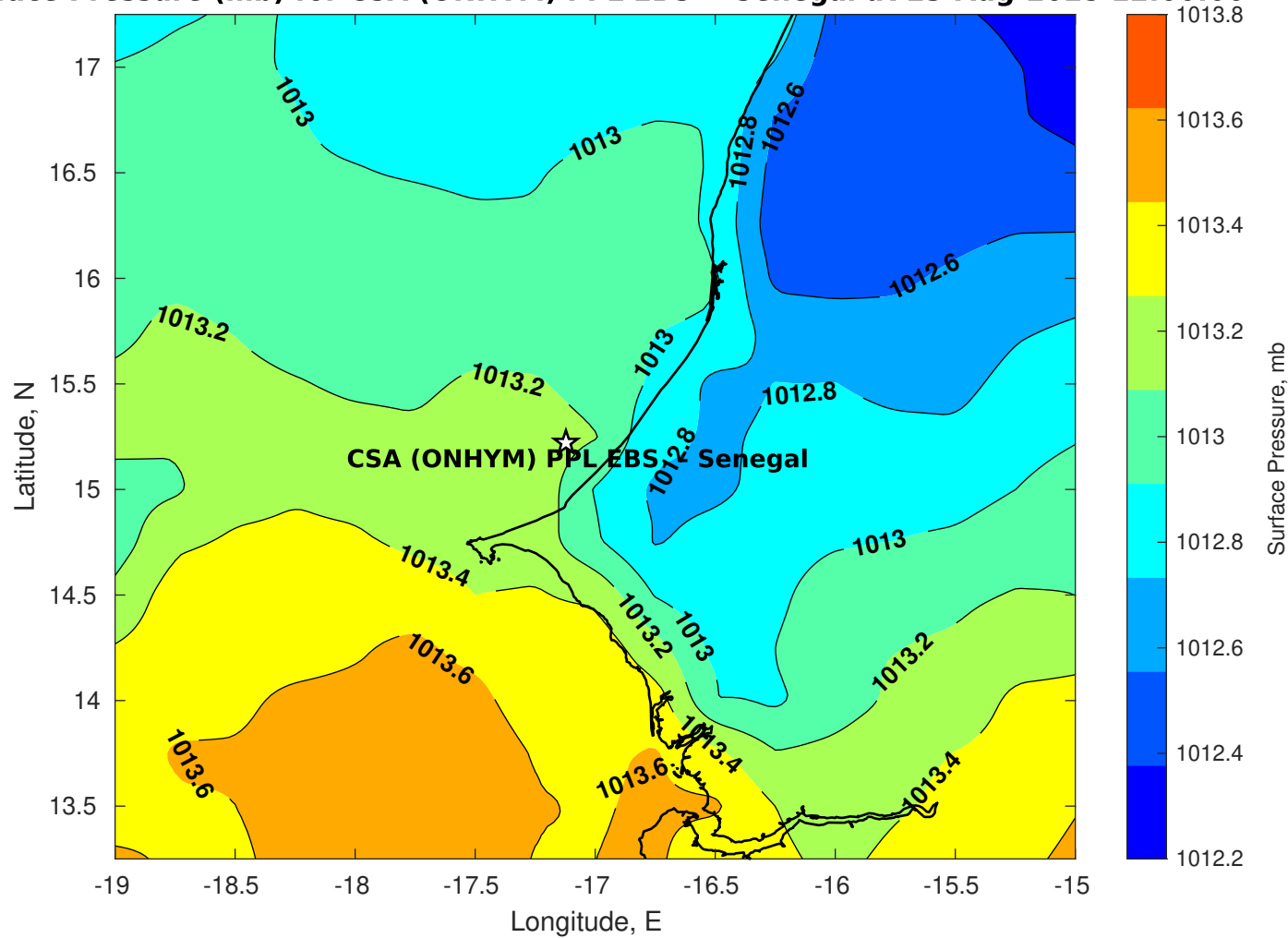
Surface Pressure (mb) for CSA (ONHYM) PPL EBS - Senegal at 23-Aug-2025 12:00:00
