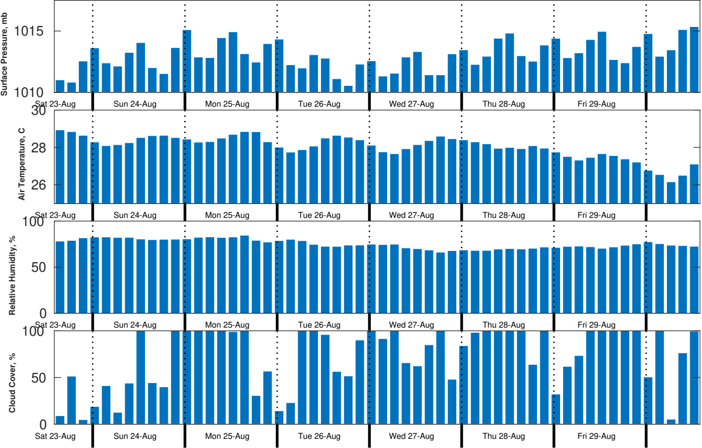
Met Forecast for CSA (ONHYM) PPL EBS - Senegal from 23-Aug-2025 12:00:00 to 30-Aug-2025 12:00:00
