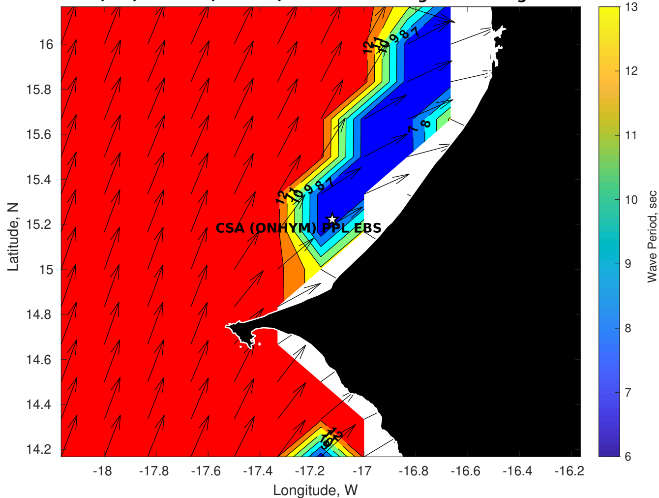
Wave Period (sec) for CSA (ONHYM) PPL EBS - Senegal at 23-Aug-2025 21:00:00
