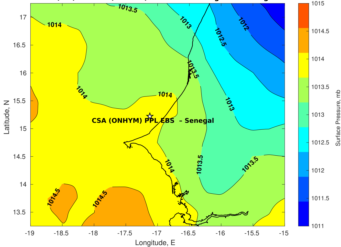
Surface Pressure (mb) for CSA (ONHYM) PPL EBS - Senegal at 24-Aug-2025 12:00:00
