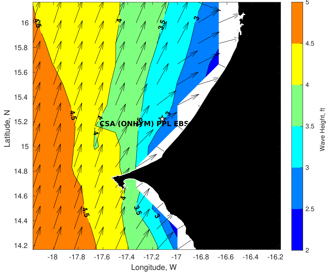
Wave Height (ft) for CSA (ONHYM) PPL EBS - Senegal at 23-Aug-2025 21:00:00
