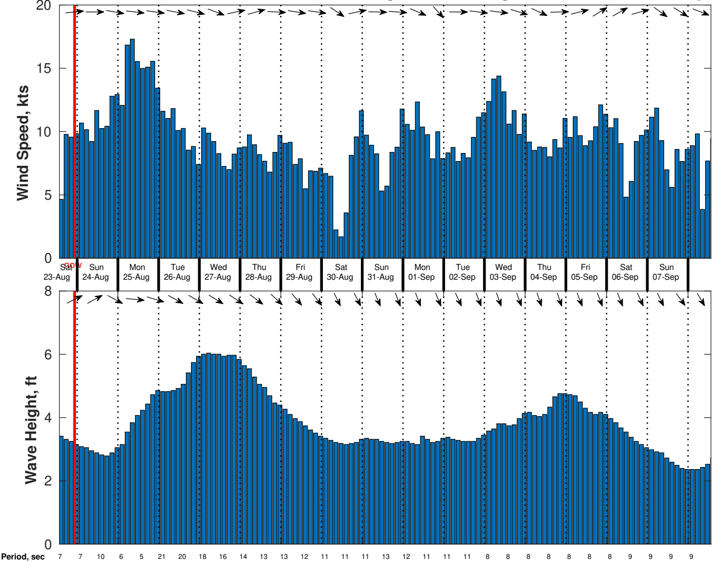
Wind & Wave Forecast for CSA (ONHYM) PPL EBS - Senegal from 23-Aug-2025 13:00:00 to 08-Sep-2025 13:00:00
