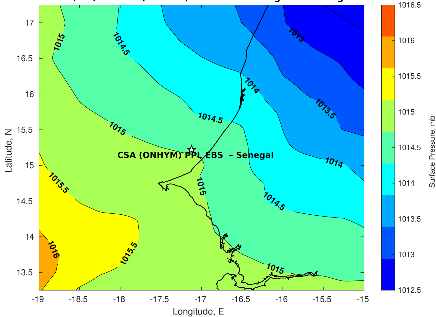
Surface Pressure (mb) for CSA (ONHYM) PPL EBS - Senegal at 25-Aug-2025 12:00:00
