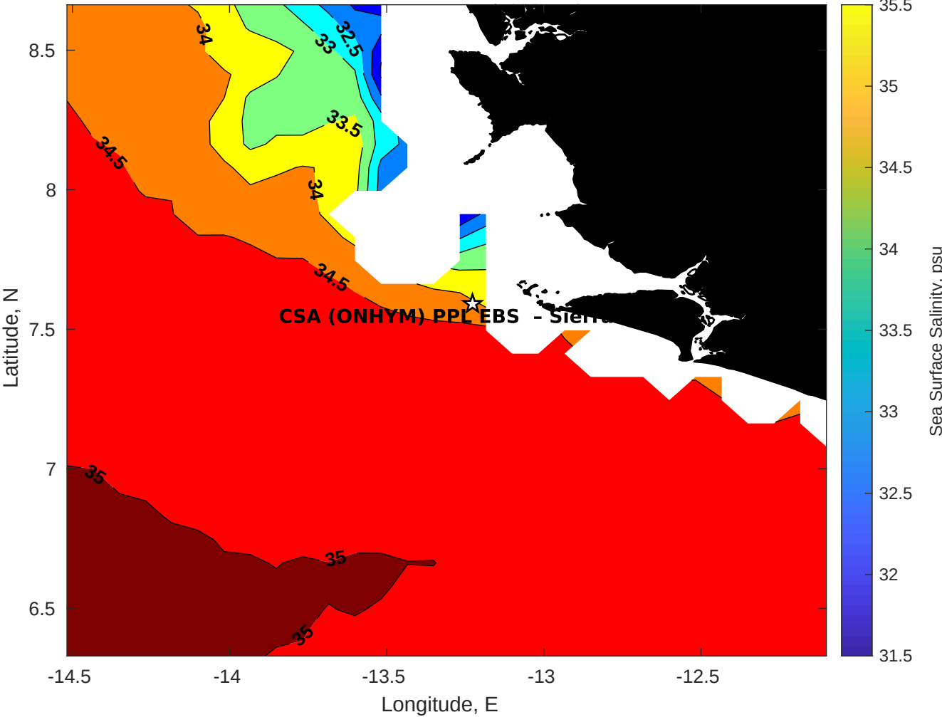
Surface Salinity for CSA (ONHYM) PPL EBS - Sierra Leone at 23-Aug-2025 00:00:00
