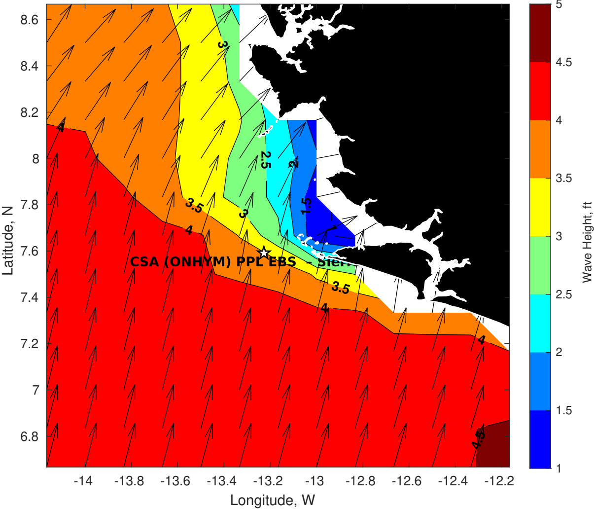
Wave Height (ft) for CSA (ONHYM) PPL EBS - Sierra Leone at 23-Aug-2025 21:00:00
