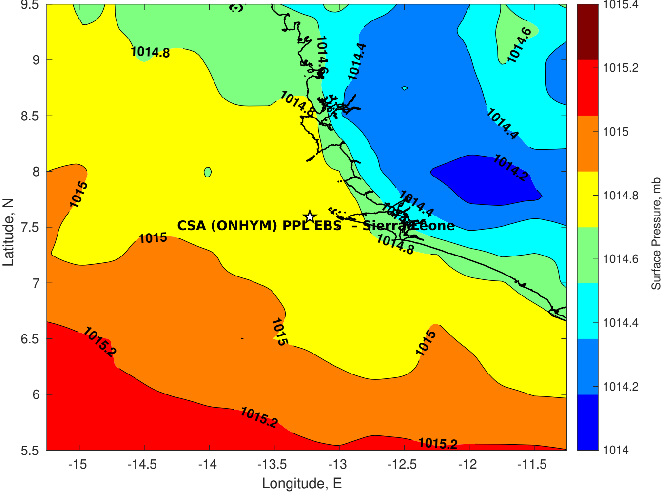
Surface Pressure (mb) for CSA (ONHYM) PPL EBS - Sierra Leone at 23-Aug-2025 12:00:00
