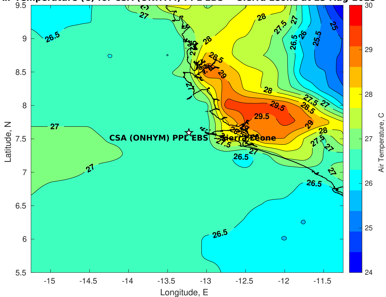
Air Temperature (C) for CSA (ONHYM) PPL EBS - Sierra Leone at 23-Aug-2025
