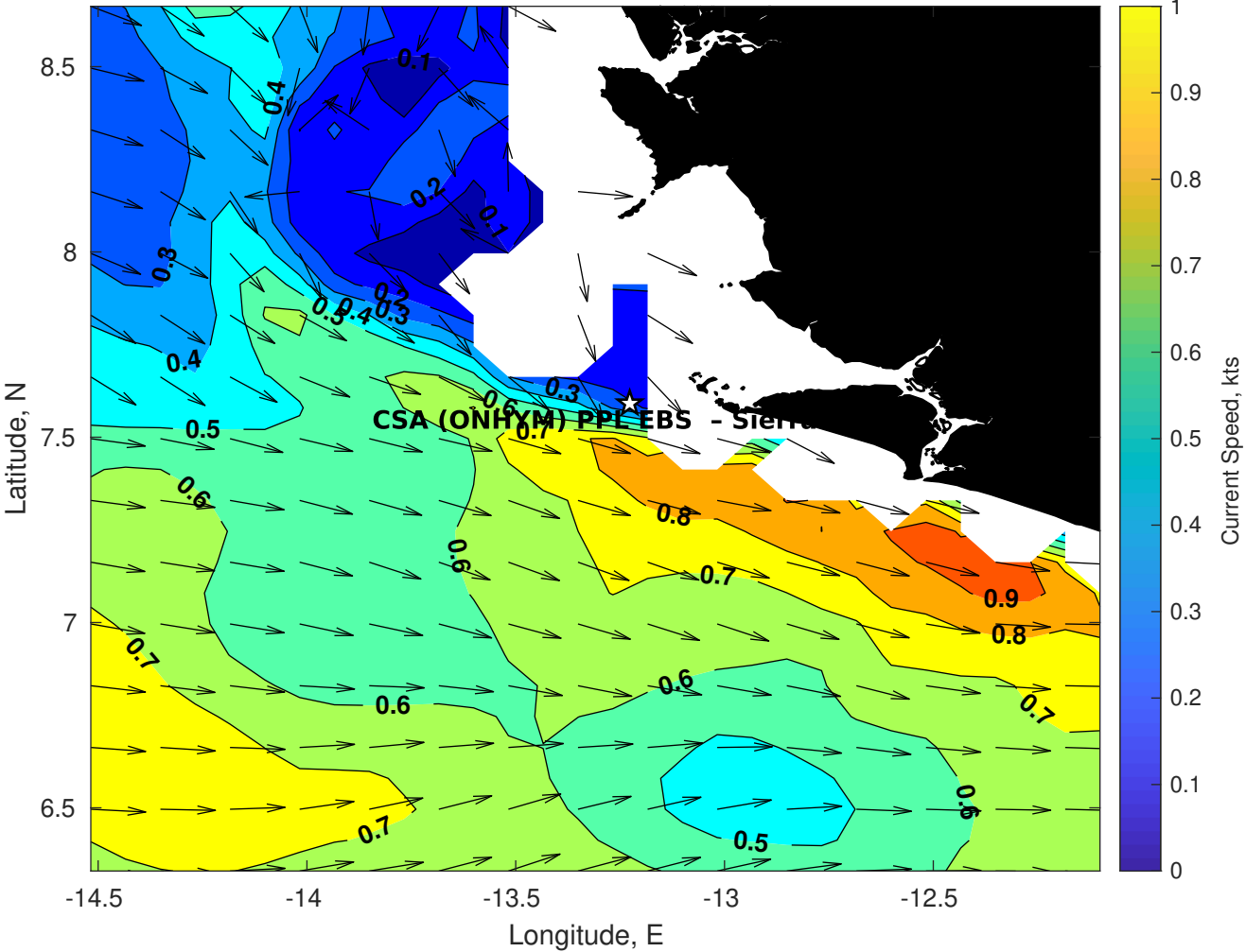
Surface Currents for CSA (ONHYM) PPL EBS - Sierra Leone at 23-Aug-2025 00:00:00
