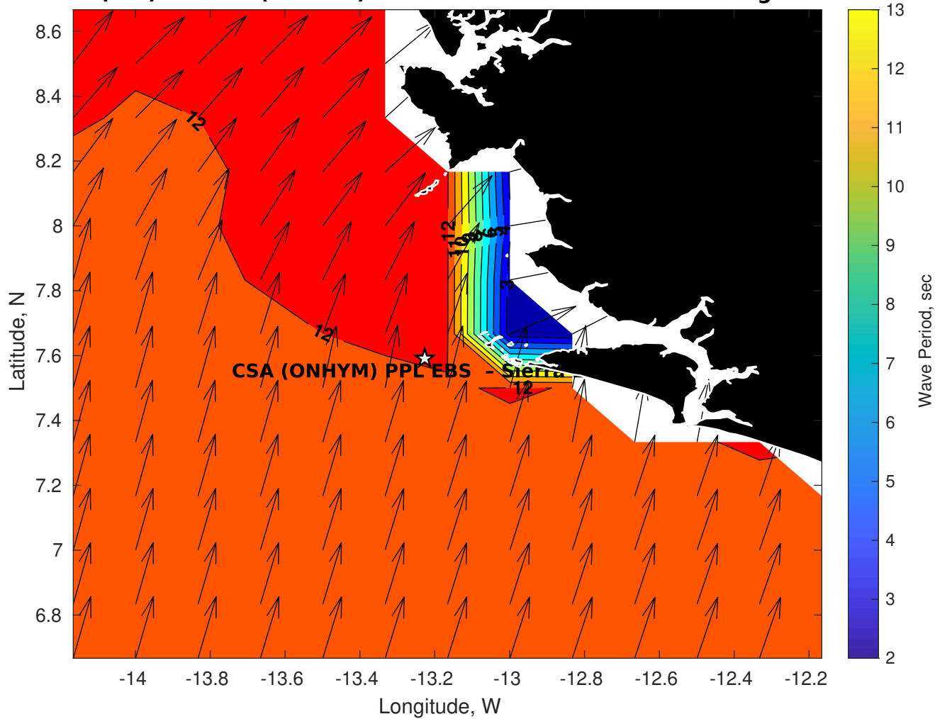
Wave Period (sec) for CSA (ONHYM) PPL EBS - Sierra Leone at 23-Aug-2025 21:00:00
