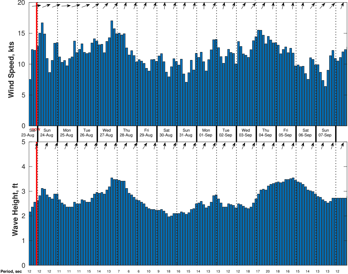
Wind & Wave Forecast for CSA (ONHYM) PPL EBS - Sierra Leone from 23-Aug-2025 13:00:00 to 08-Sep-2025 13:00:00
