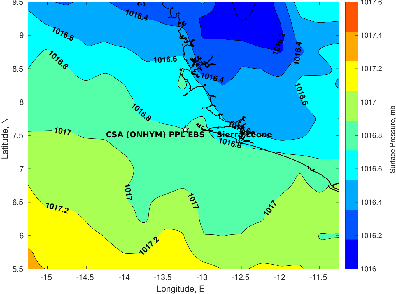
Surface Pressure (mb) for CSA (ONHYM) PPL EBS - Sierra Leone at 25-Aug-2025 12:00:00
