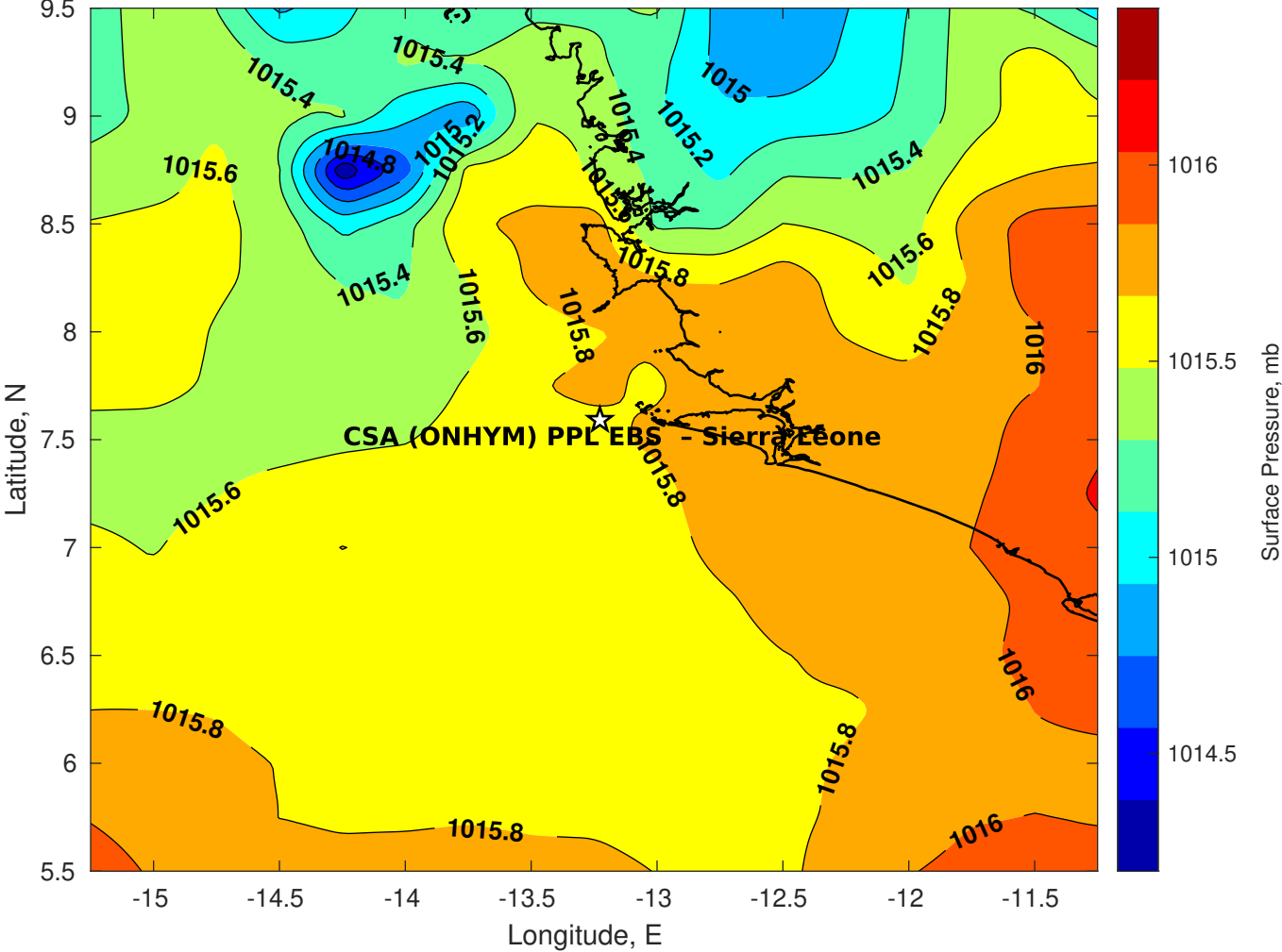
Surface Pressure (mb) for CSA (ONHYM) PPL EBS - Sierra Leone at 24-Aug-2025 12:00:00
