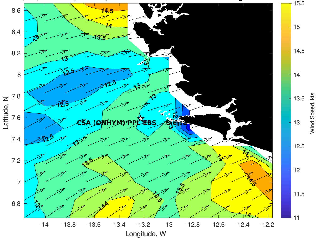
Winds (kts) for CSA (ONHYM) PPL EBS - Sierra Leone at 23-Aug-2025 21:00:00
