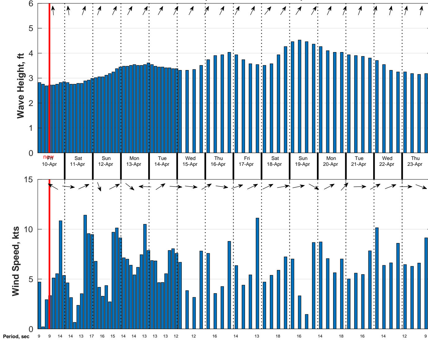
Wind & Wave Forecast for Liberia from 09-Apr-2026 01:00:00 to 23-Apr-2026 01:00:00
