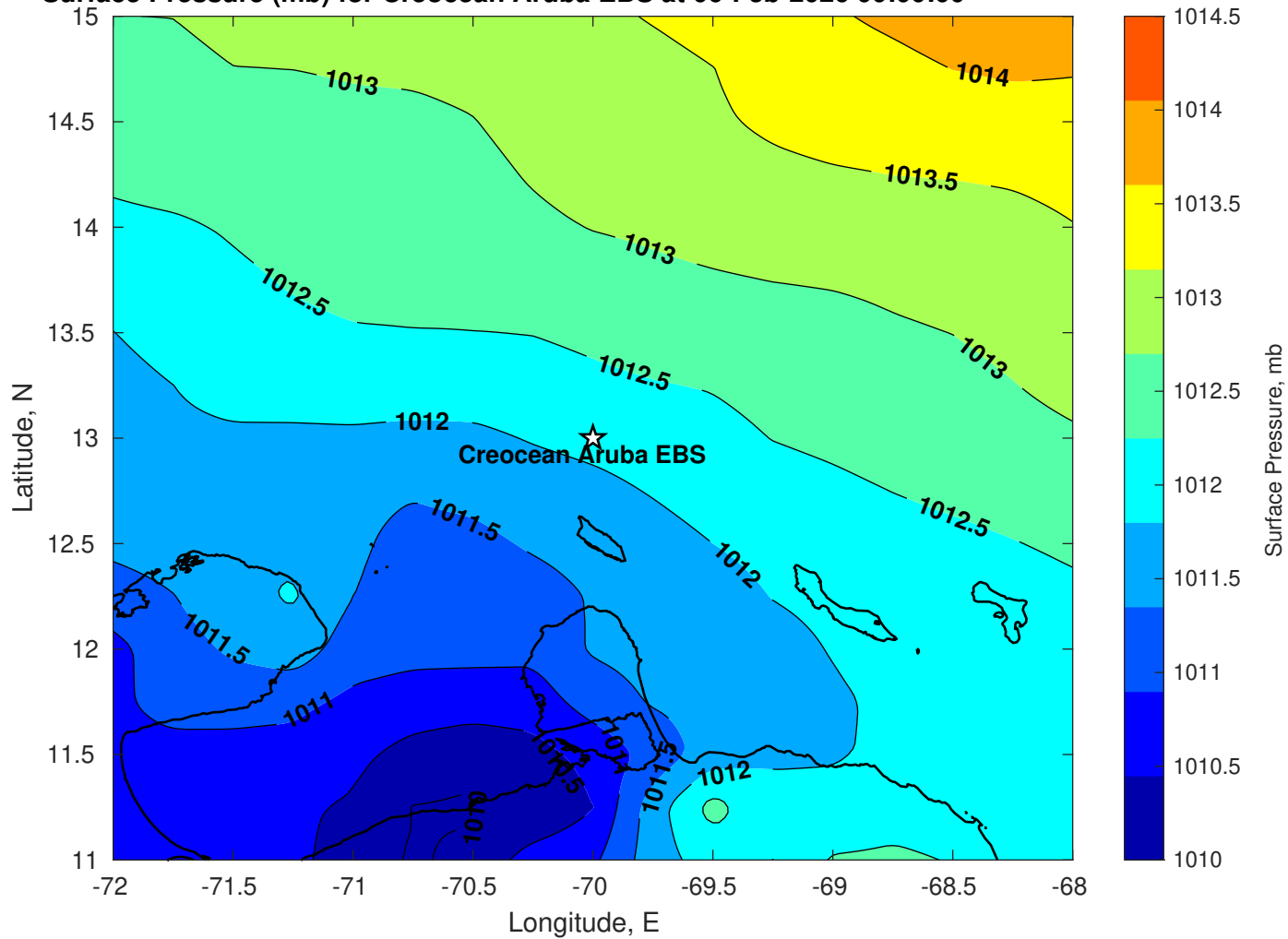
Surface Pressure (mb) for Creoccean Aruba EBS at 06-Feb-2026 00:00:00
