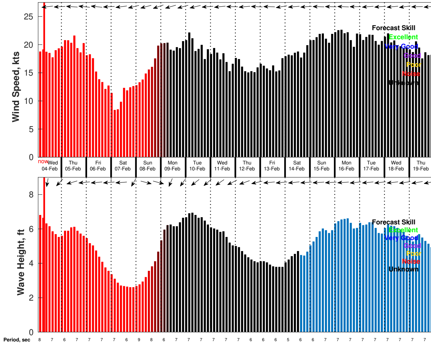
Wind & Wave Forecast for Creocan Aruba EBS from 04-Feb-2026 02:00:00 to 20-Feb-2026 02:00:00
