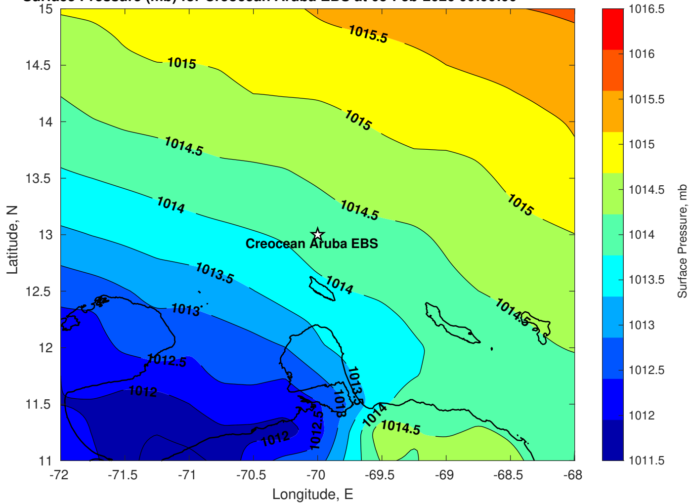
Surface Pressure (mb) for Creoccean Aruba EBS at 05-Feb-2026 00:00:00
