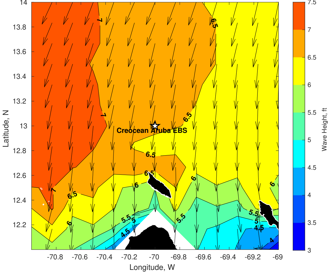
GFS Wave Height (ft) for Creoccean Aruba EBS at 04-Feb-2026 09:00:00
