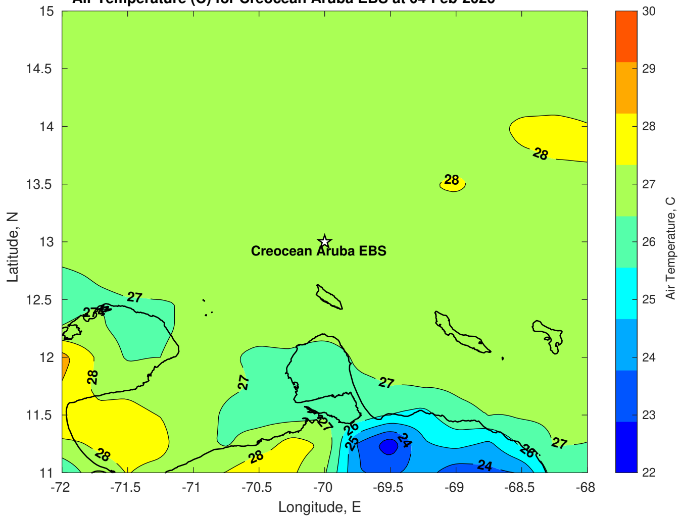
Air Temperature (C) for Creoccean Aruba EBS at 04-Feb-2026
