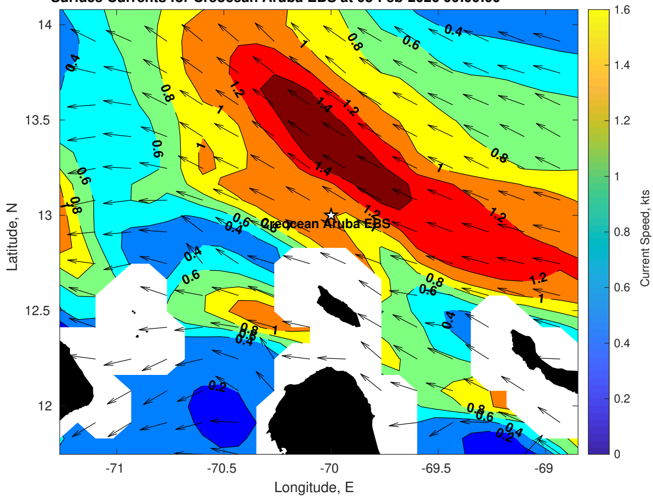
Surface Currents for Crecean Aruba EBS at 03-Feb-2026 00:00:00
