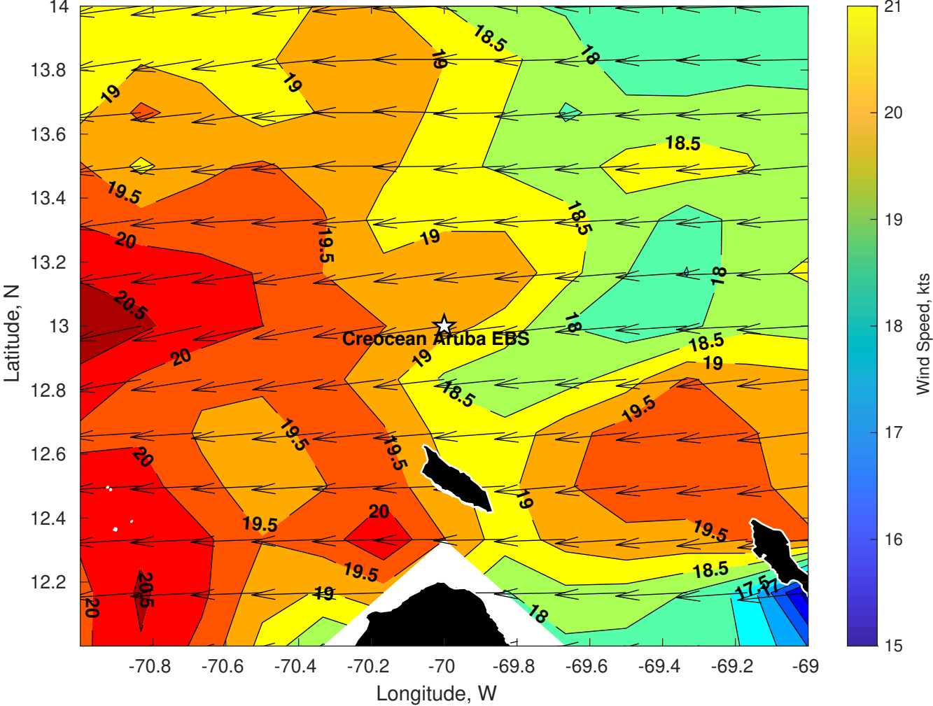
GFS Winds (kts) for Creoccean Aruba EBS at 04-Feb-2026 09:00:00
