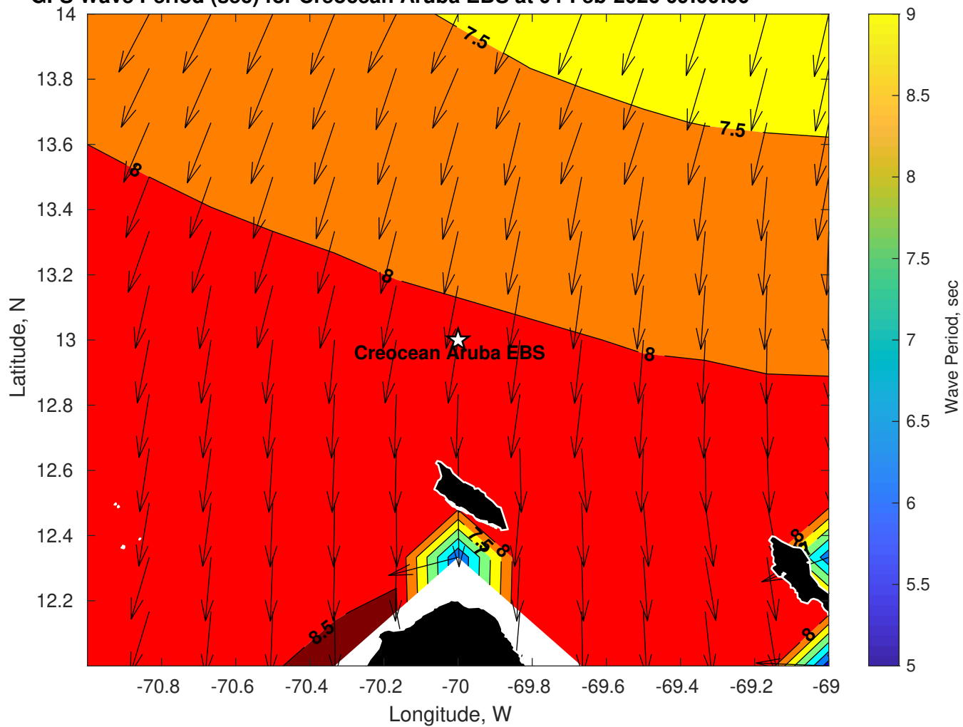
GFS Wave Period (sec) for Creoccean Aruba EBS at 04-Feb-2026 09:00:00
