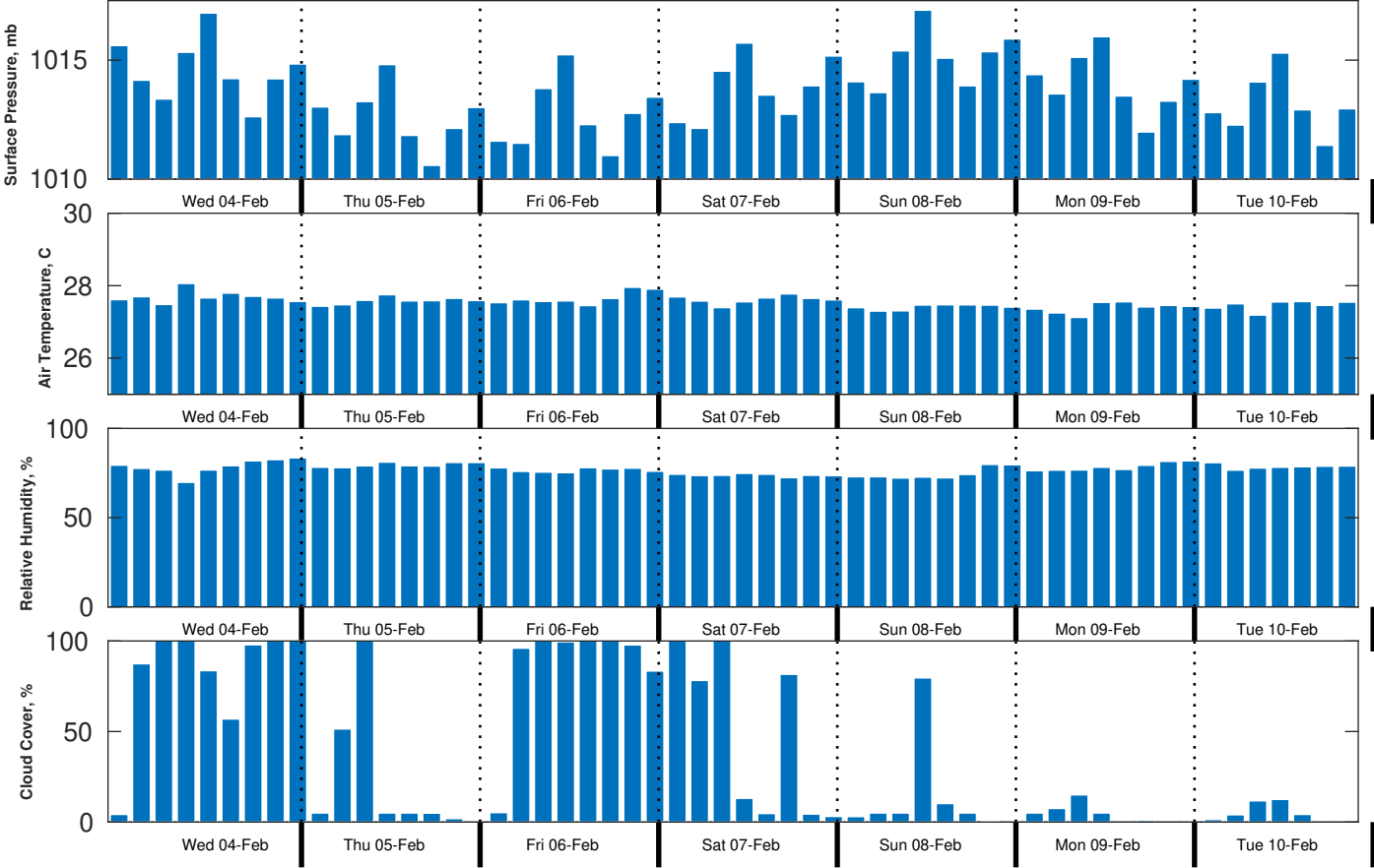
Met Forecast for Creocan Aruba EBS from 04-Feb-2026 00:00:00 to 11-Feb-2026 00:00:00
