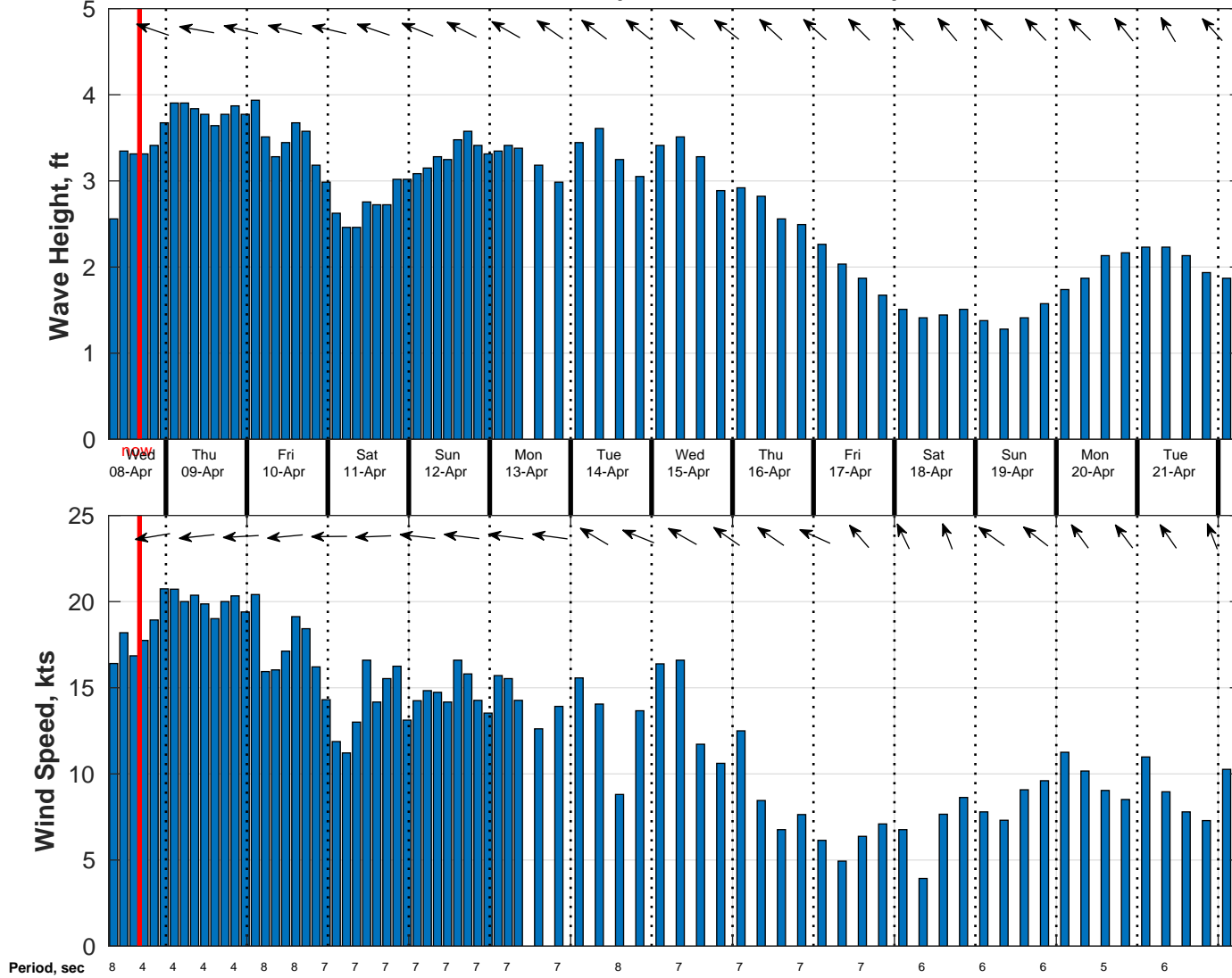
Wind & Wave Forecast for NDBC 42084 from 08-Apr-2026 07:00:00 to 22-Apr-2026 07:00:00
