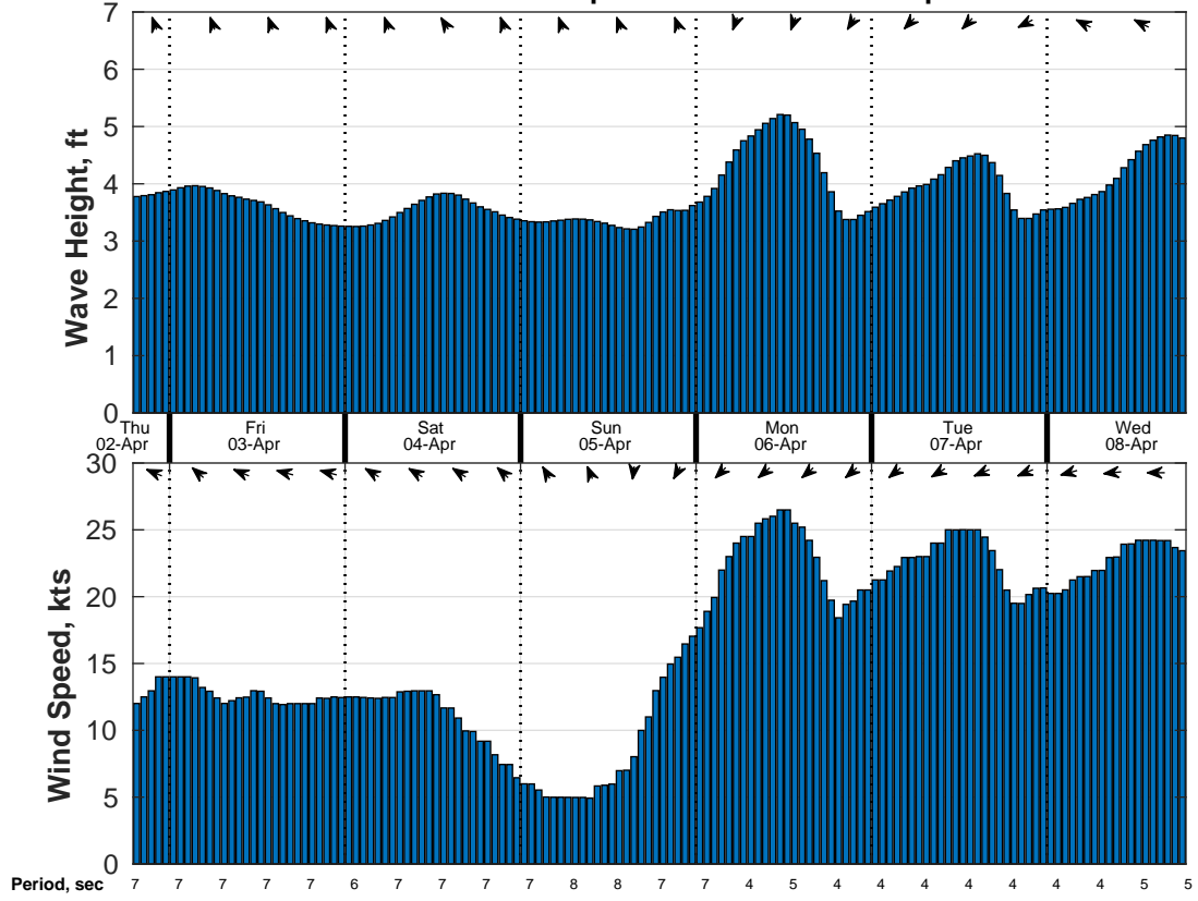
Wind & Wave Forecast for NDBC 42084 from 02-Apr-2026 19:00:00 to 08-Apr-2026 19:00:00
