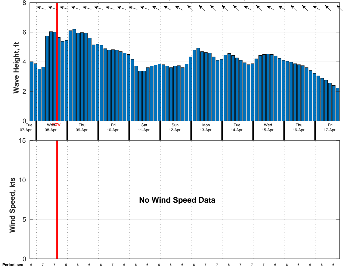
Wind & Wave Forecast for NDBC 42084 from 07-Apr-2026 19:00:00 to 17-Apr-2026 19:00:00
