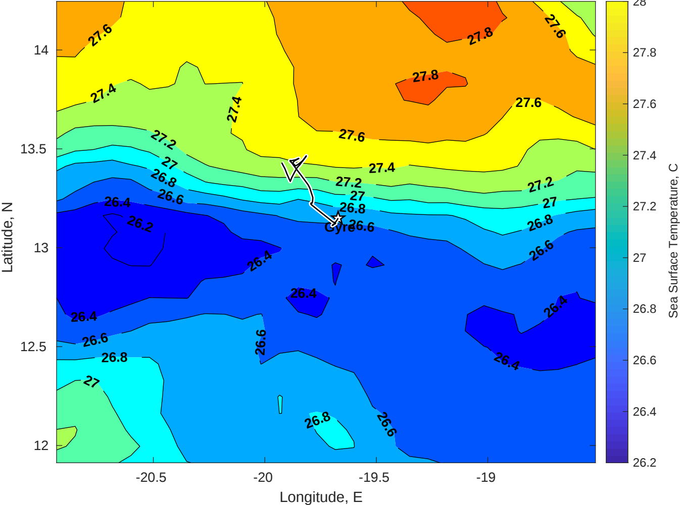
SST for Gyre at 23-Aug-2025 00:00:00
