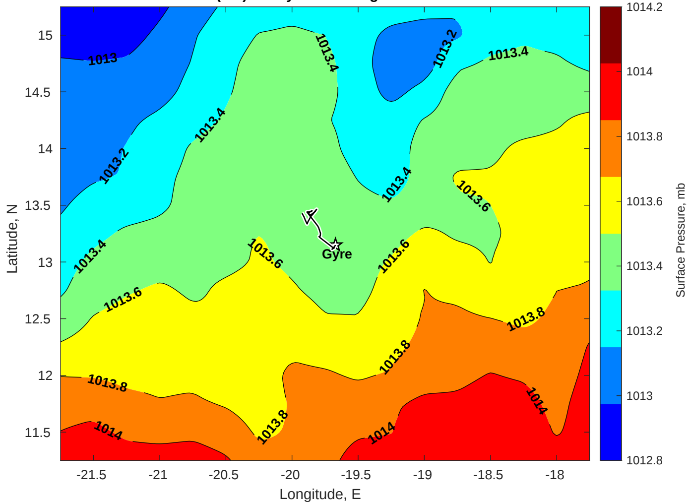
Surface Pressure (mb) for Gyre at 23-Aug-2025 12:00:00
