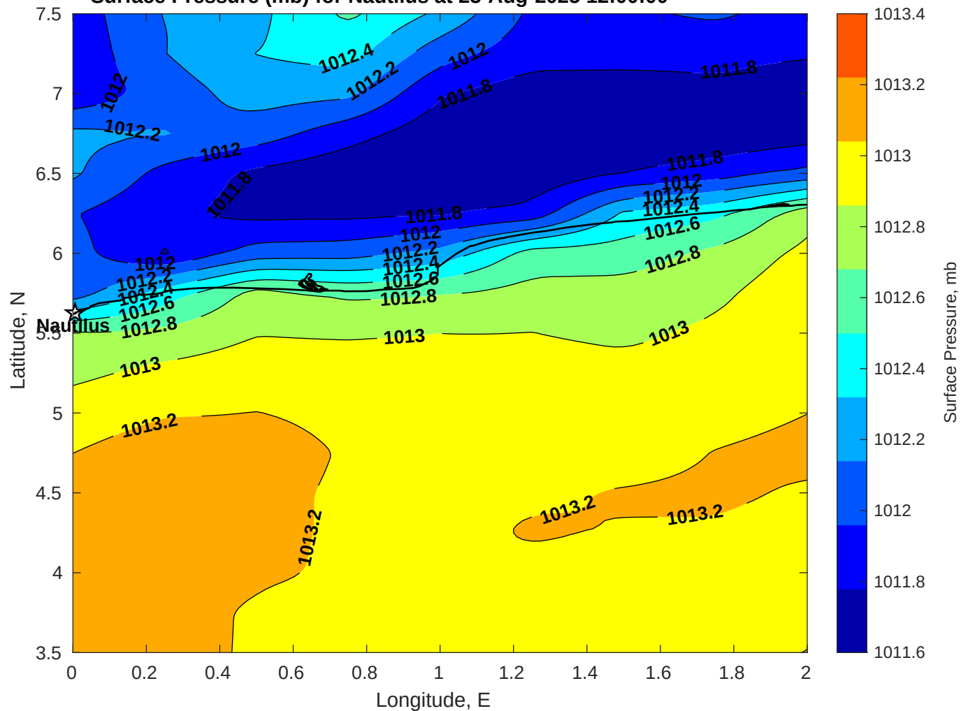
Surface Pressure (mb) for Nautilus at 23-Aug-2025 12:00:00
