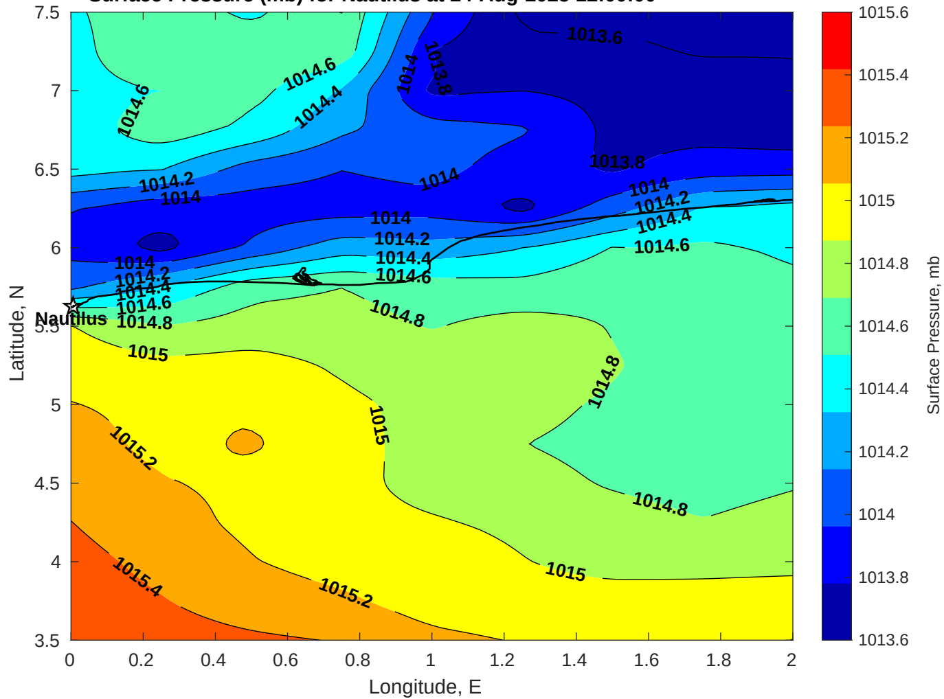
Surface Pressure (mb) for Nautilus at 24-Aug-2025 12:00:00
