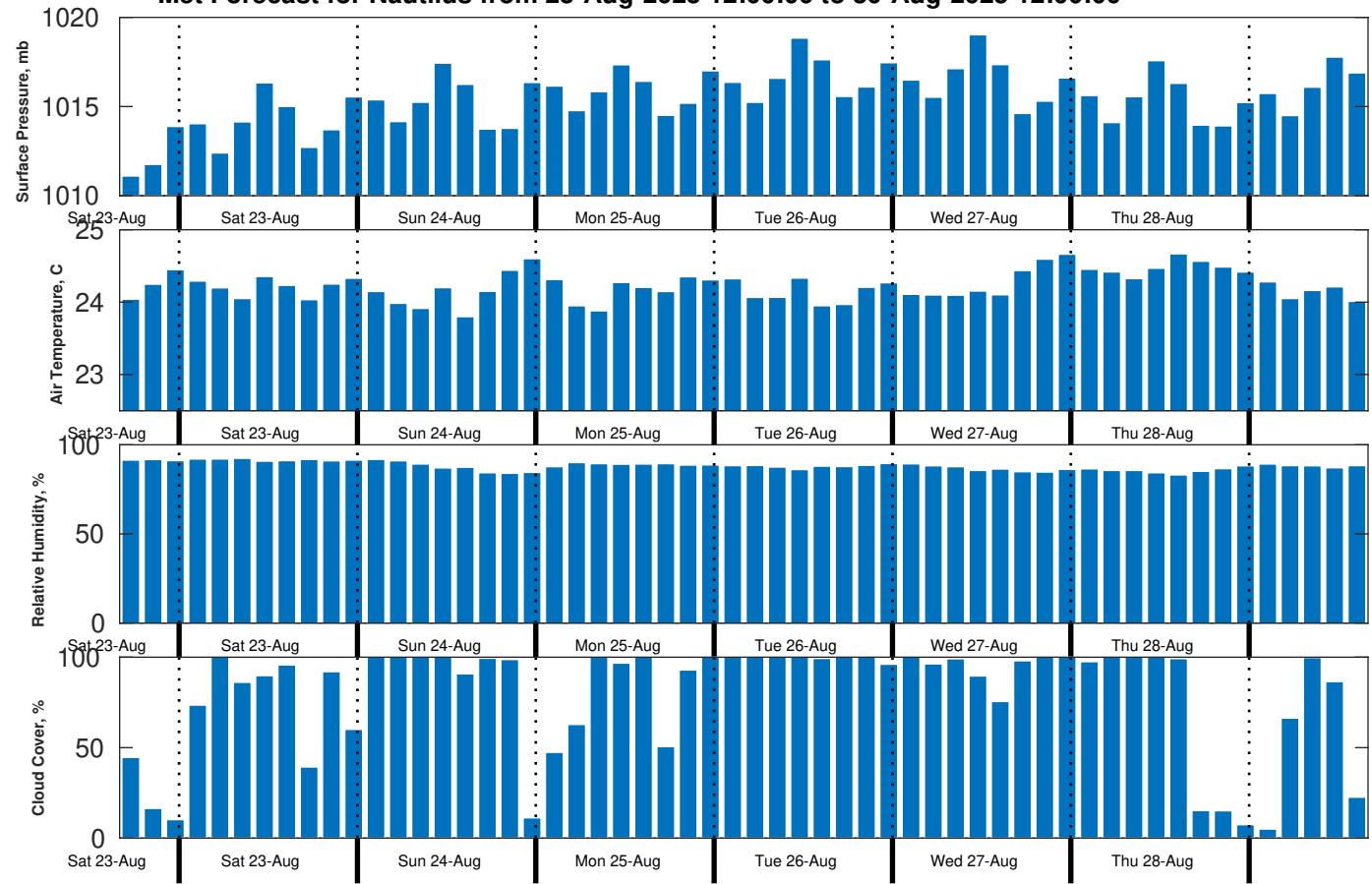
Met Forecast for Nautilus from 23-Aug-2025 12:00:00 to 30-Aug-2025 12:00:00
