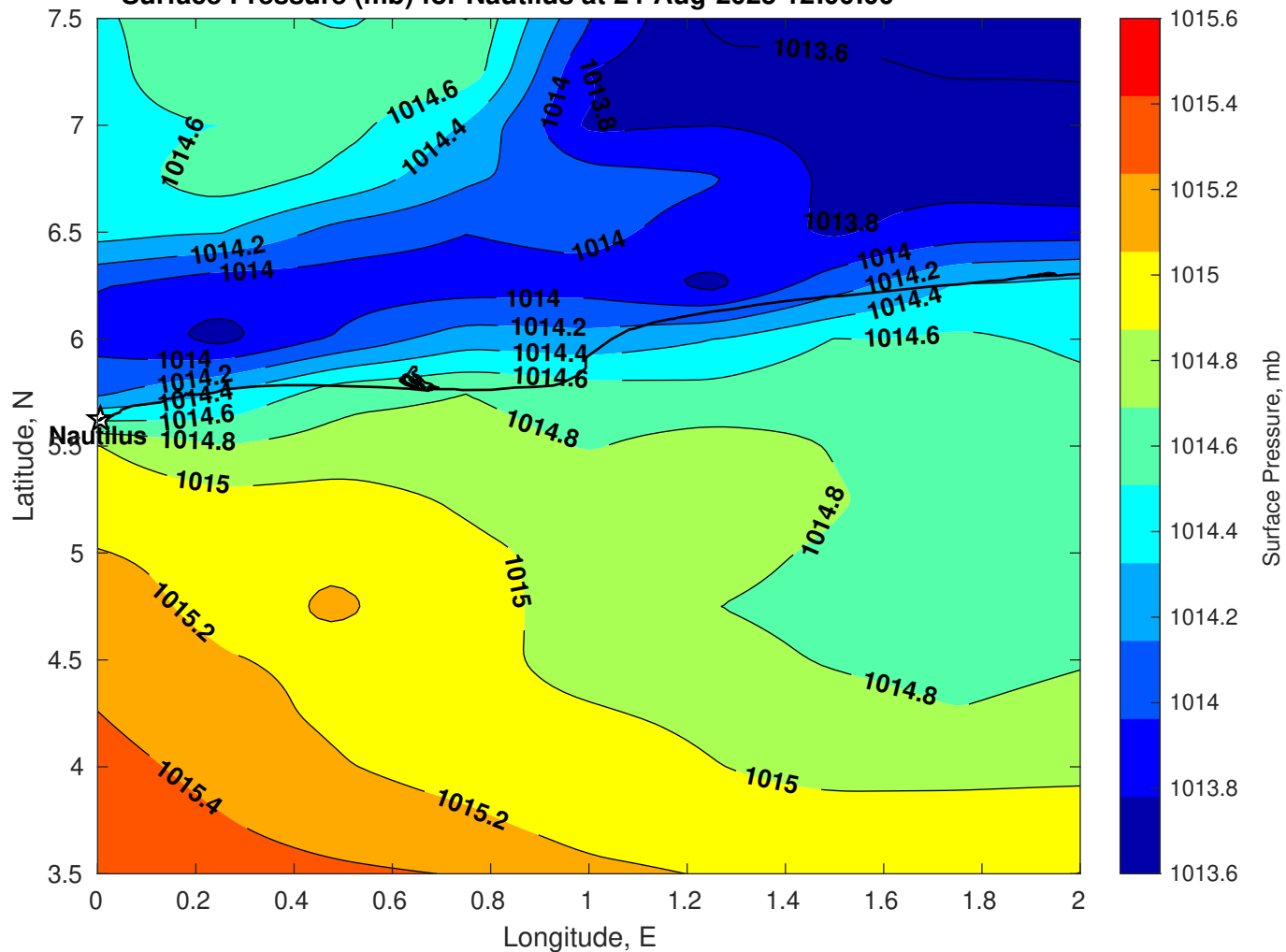
Surface Pressure (mb) for Nautilus at 24-Aug-2025 12:00:00
