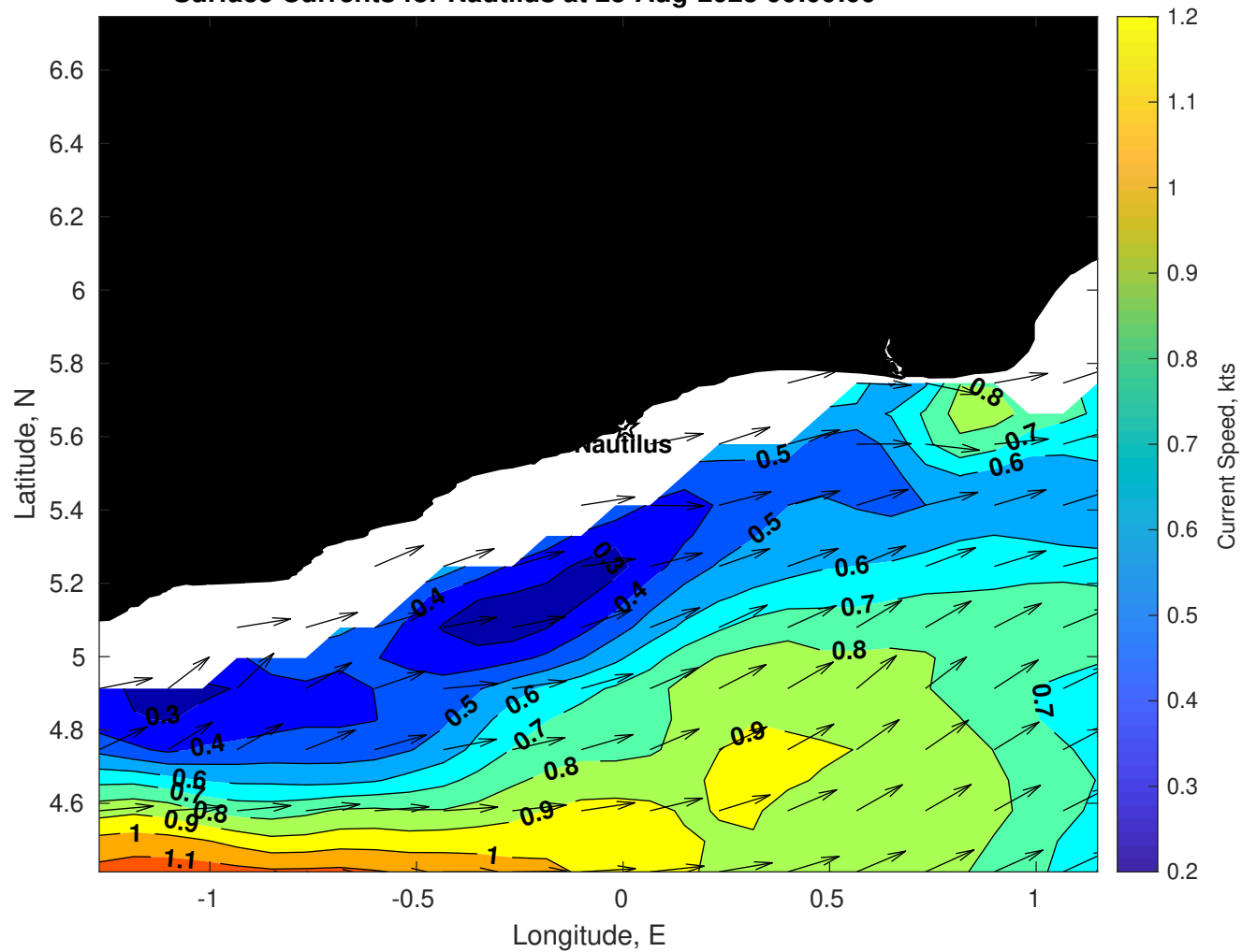
Surface Currents for Nautilus at 23-Aug-2025 00:00:00
