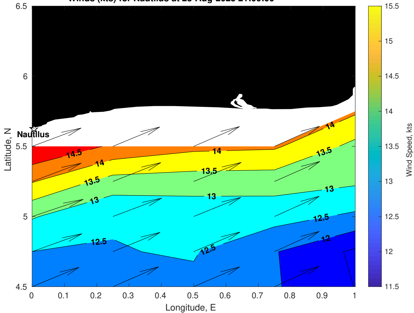
Winds (kts) for Nautilus at 23-Aug-2025 21:00:00
