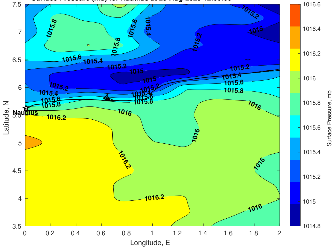
Surface Pressure (mb) for Nautilus at 25-Aug-2025 12:00:00
