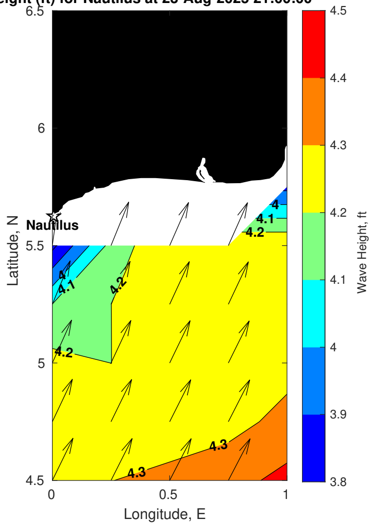
Wave Height (ft) for Nautilus at 23-Aug-2025 21:00:00
