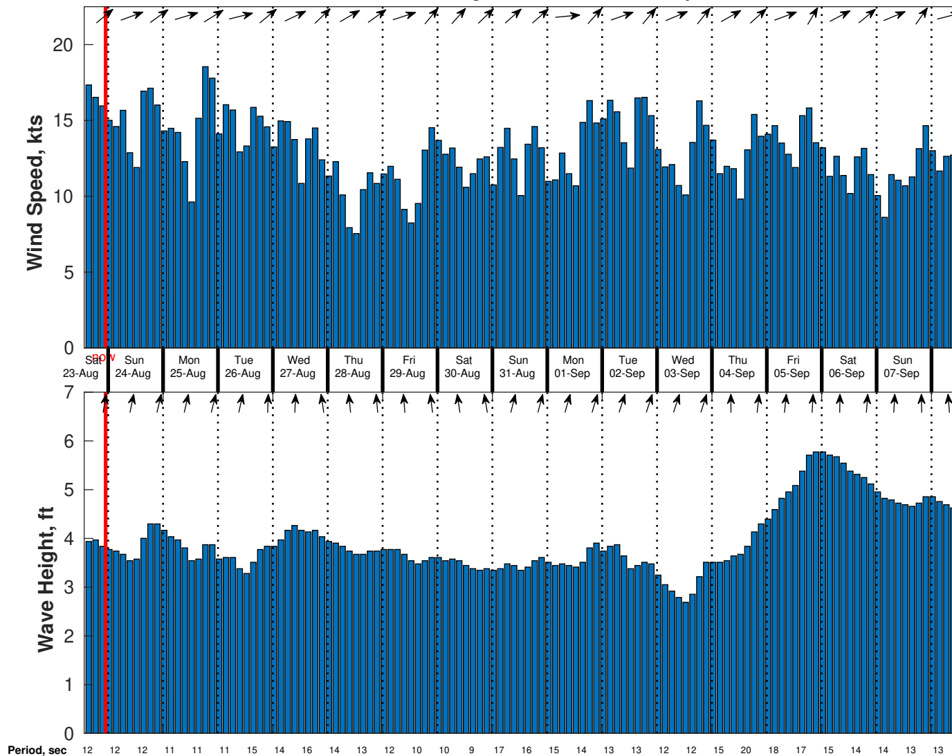
Wind & Wave Forecast for Nautilus from 23-Aug-2025 14:00:00 to 08-Sep-2025 14:00:00
