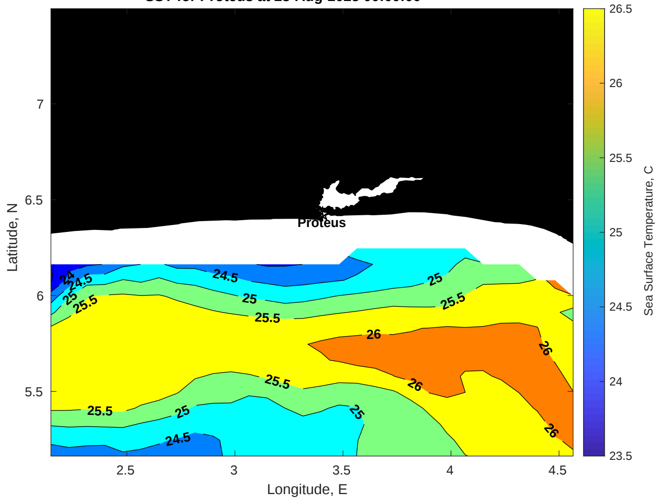
SST for Proteus at 23-Aug-2025 00:00:00
